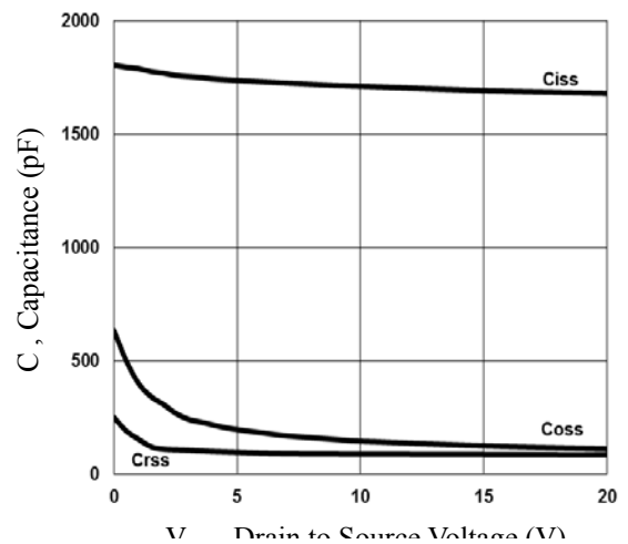
Fig.6 Capacitance Characteristics
