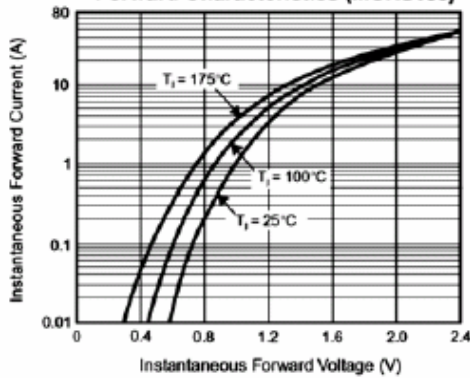
Fig. 3 – Typical Instantaneous Forward Characteristics (MURS160)
