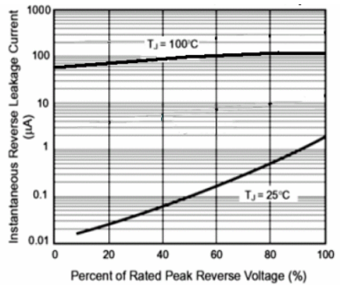
Fig. 4 – Typical Reverse Leakage Characteristics (MURS160)
