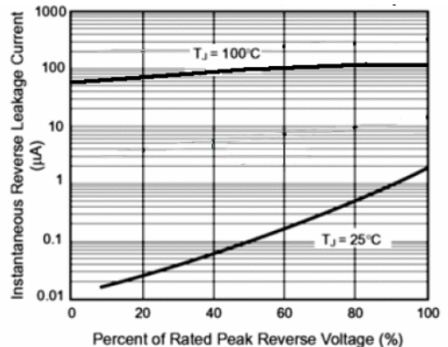
Fig. 4 – Typical Reverse Leakage Characteristics (MURS160)
