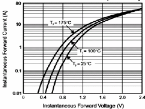
Fig. 3 – Typical Instantaneous Forward Characteristics (MURS160)
