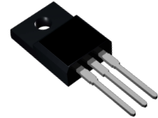
MBRF3045CT Package: ITO-220-AB
