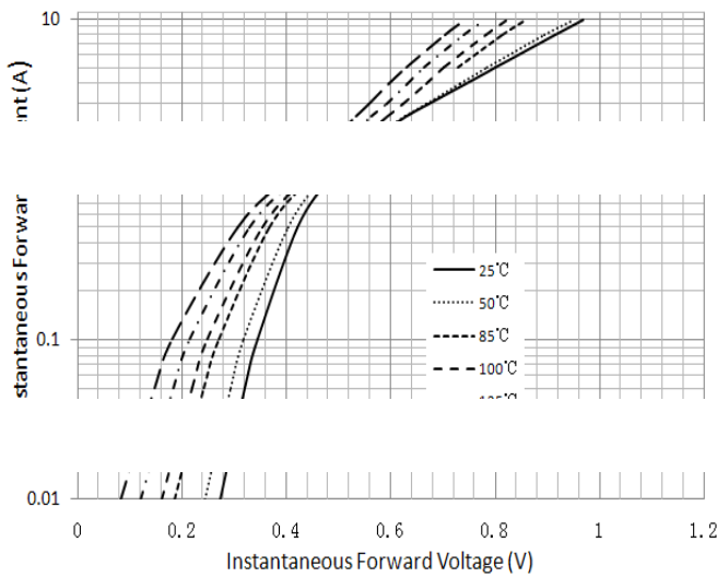
Figure 1. Typical Instantaneous Forward Characteristics
