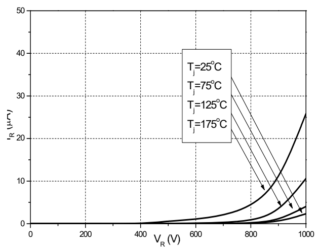
Figure 2. Reverse Characteristics
