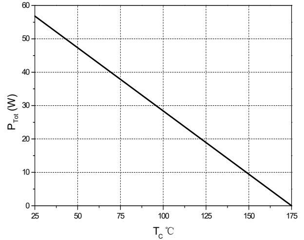
Figure 6. Power Derating
