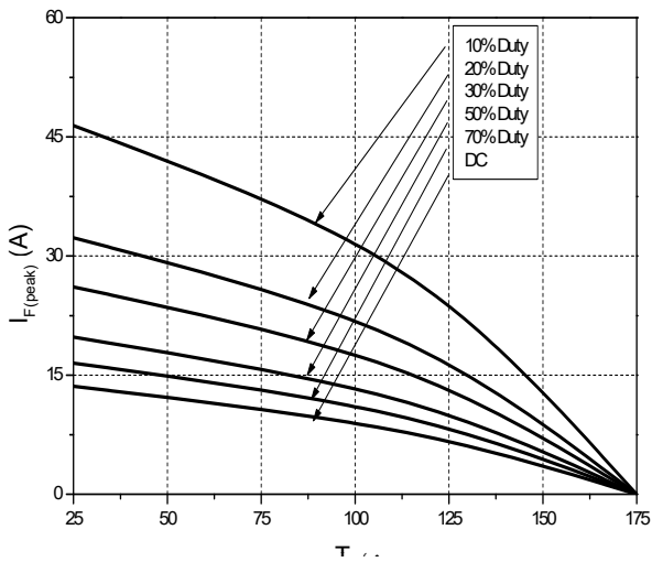
Figure 7. Current Derating
