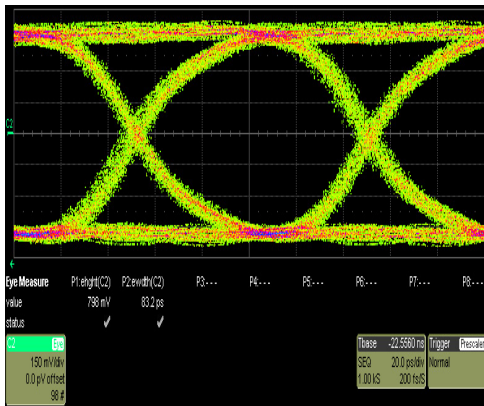
Fig.3 Eye Diagram - USB3.1 at 10Gbps per channel (with SPESUC5VD2010-5U)
