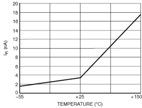
Fig 2. Typical Leakage Current versus Temperature
