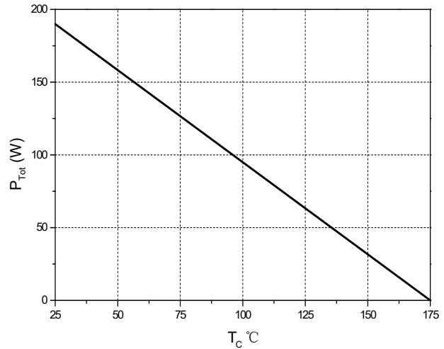
Figure 6. Power Derating
