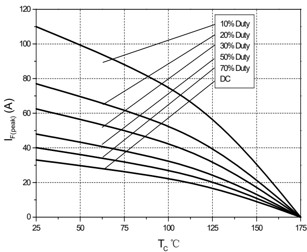
Figure 7. Current Derating
