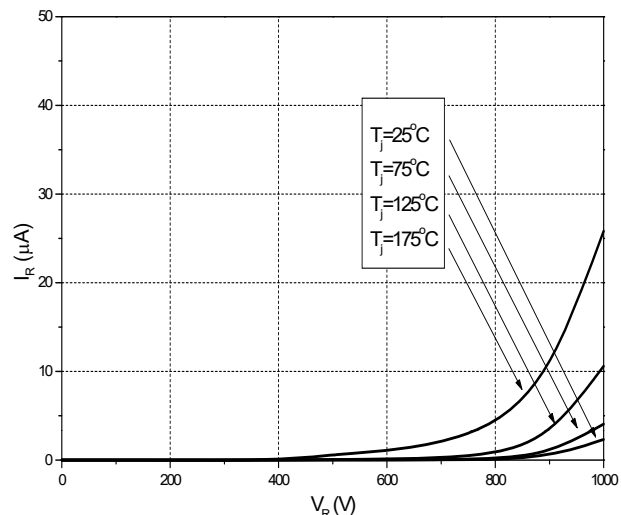
Figure 2. Reverse Characteristics
