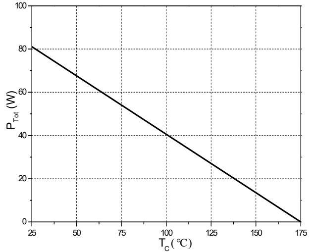
Figure 6. Power Derating
