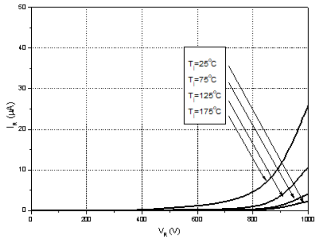
Figure 2. Reverse Characteristics
