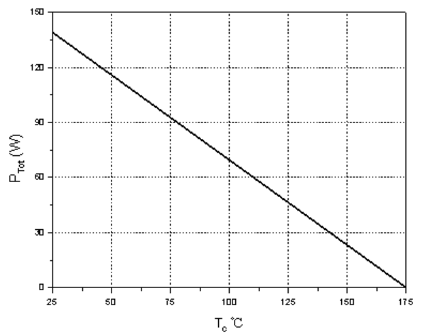
Figure 6. Power Derating
