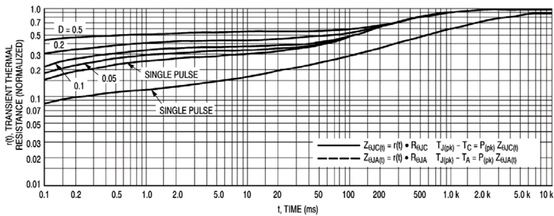
Figure 12. Thermal Response
