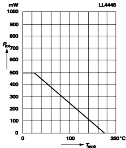
Admissible power dissipation versus ambient temperature
