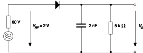
Rectification Efficiency Measurement Circuit
