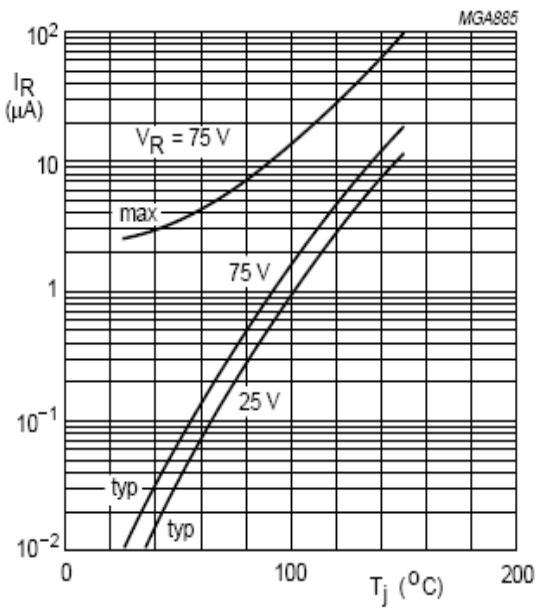
Figure 4. Reverse Current
