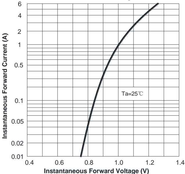
FIG3: Forward Voltage
