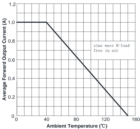
FIG1:Io-Ta Curve
