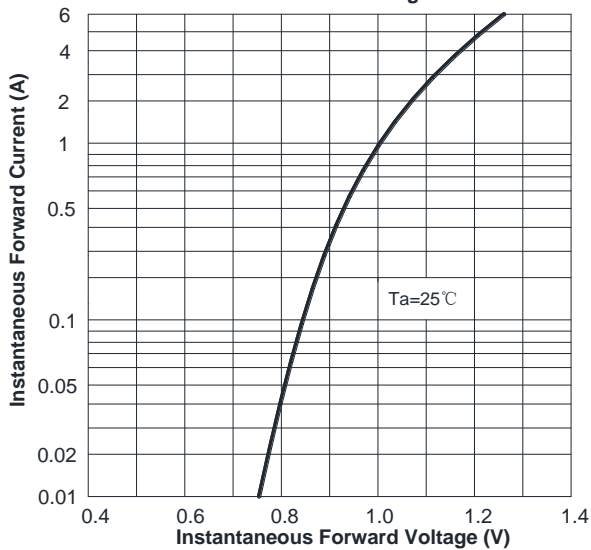
FIG3: Forward Voltage
