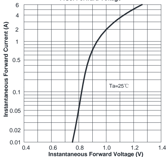
FIG3: Forward Voltage
