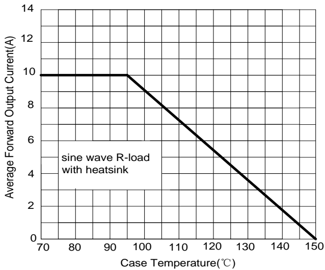
FIG1:Io-Tc Curve
